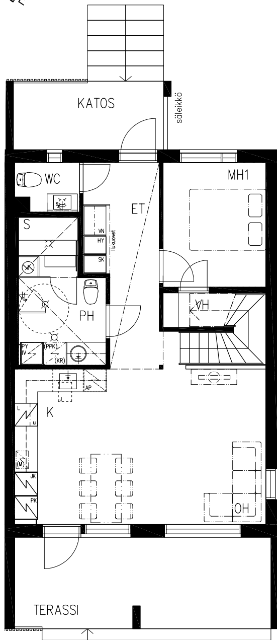
1. krs
